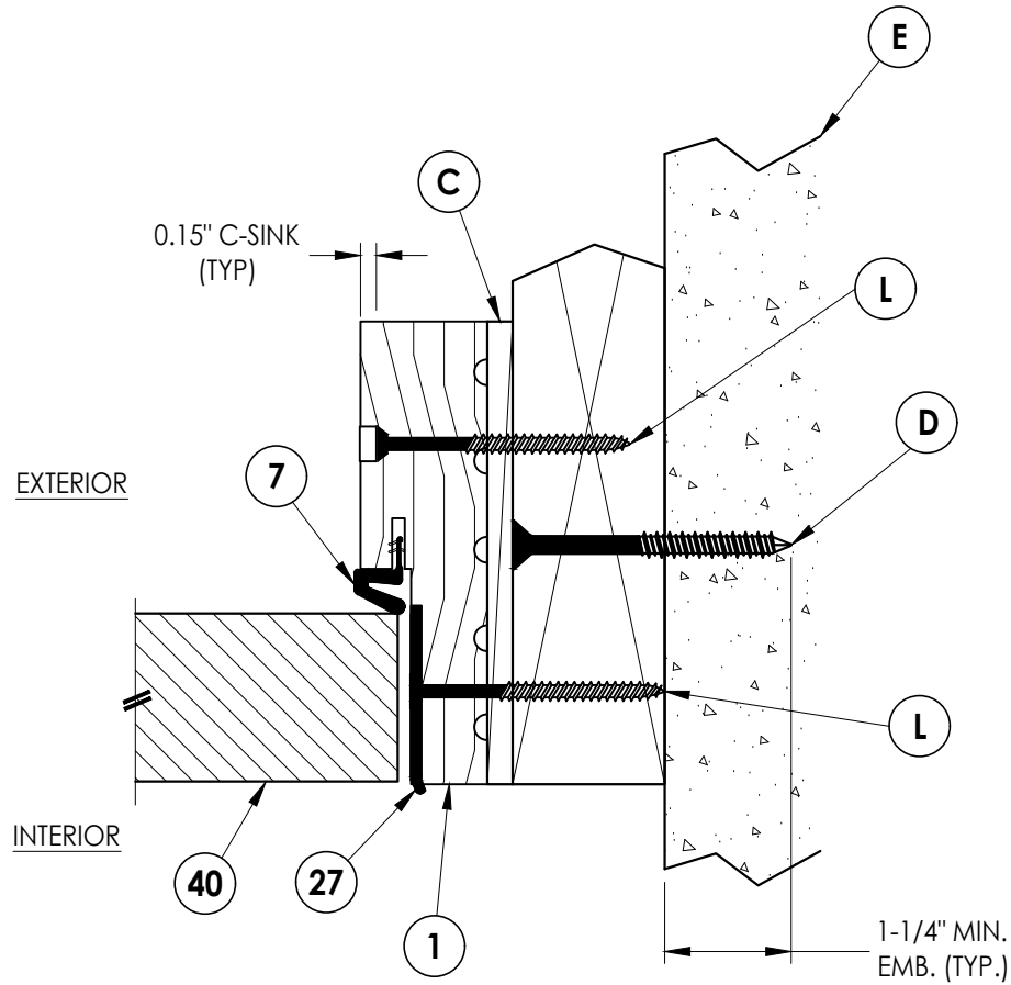
2 4 HORIZONTAL CROSS SECTION Shown w/ 2X Buck Inswing shown (Outswing similar)
