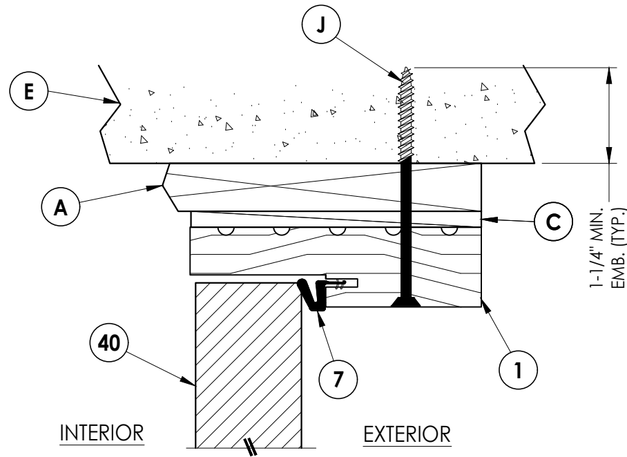
3 5 VERTICAL CROSS SECTION Shown w/ 1X sub-buck Inswing shown (Outswing similar)
