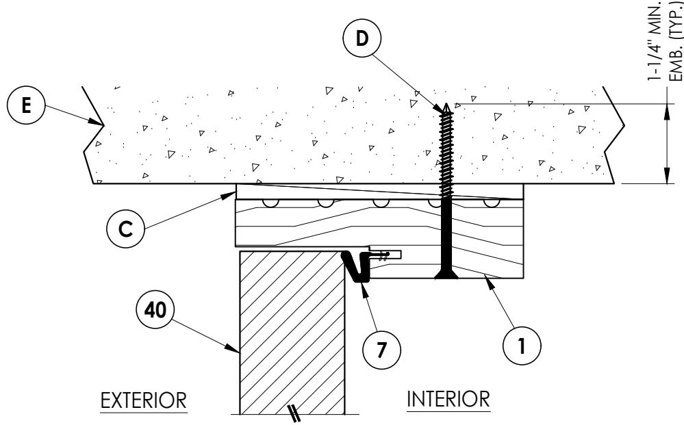
3 6 VERTICAL CROSS SECTION Shown Direct to Masonry Outswing only
