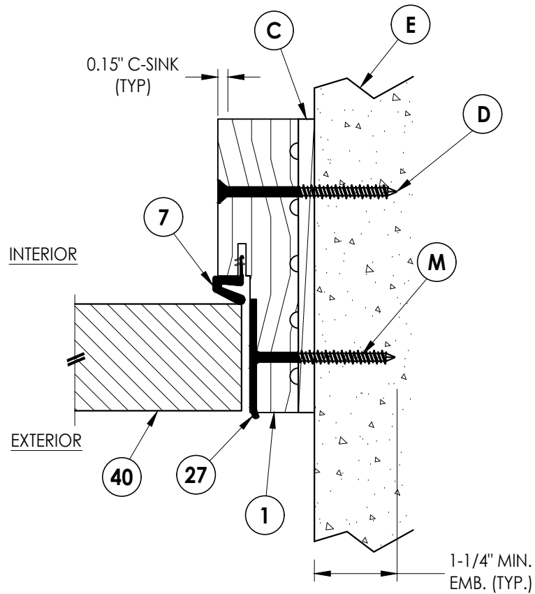
2 6 HORIZONTAL CROSS SECTION Shown Direct to Masonry Outswing only
