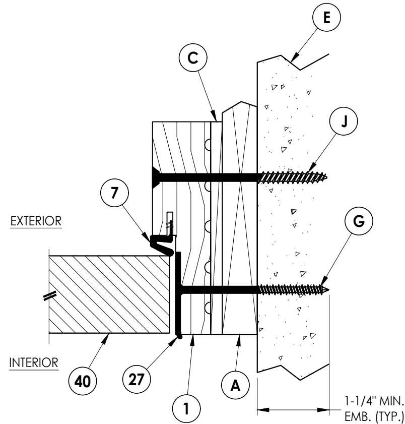
2 5 HORIZONTAL CROSS SECTION Shown w/ 1X sub-buck Inswing shown (Outswing similar)
