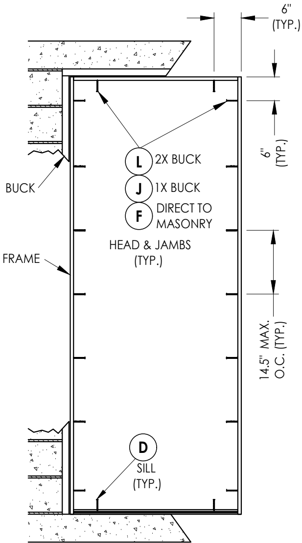
FRAME ANCHORING
